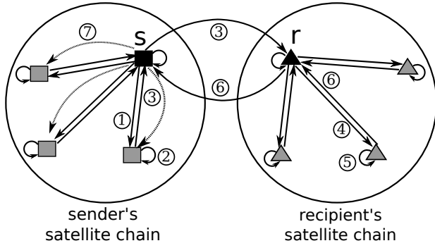
Figure 2: Atomic asset transfer between the sender node ( s ) and recipient node ( r ) across two satellite chains: ① s issues transfer transaction; ② nodes verify and execute transfer; ③ s aggregates authenticated approvals on transfer and forwards to r ; ④ r issues \text{transfer}_f transaction; ⑤ nodes verify and execute \text{transfer}_f ; ⑥ r aggregates authenticated approvals on either receipt or reject and sends back; ⑦ s issues \text{reject}_f to restore account in case the transaction fails in the recipient’s chain.
